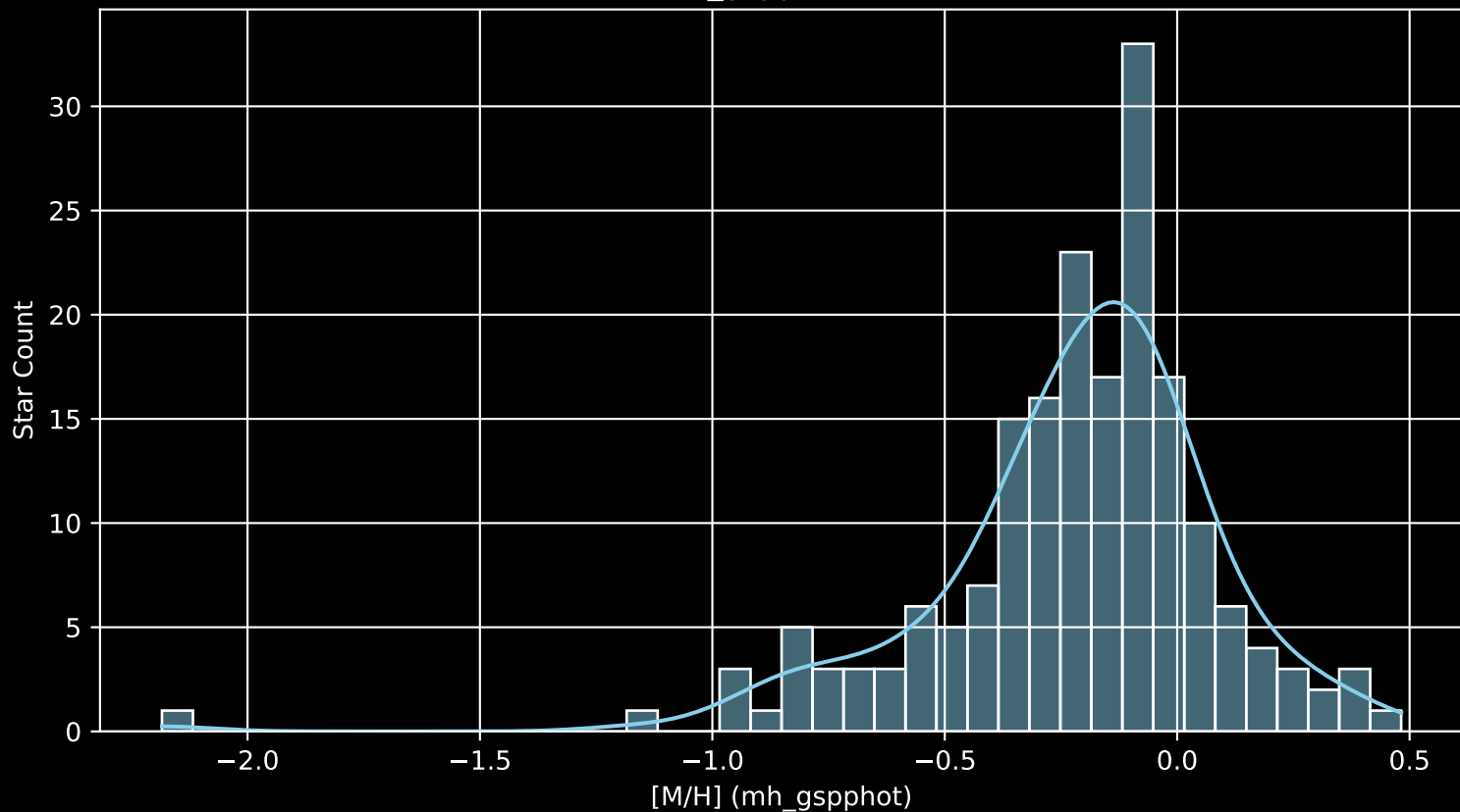
APOGEE DR17 Field: [261+48 [M/H] (mh_gspphot) (n= 188)
