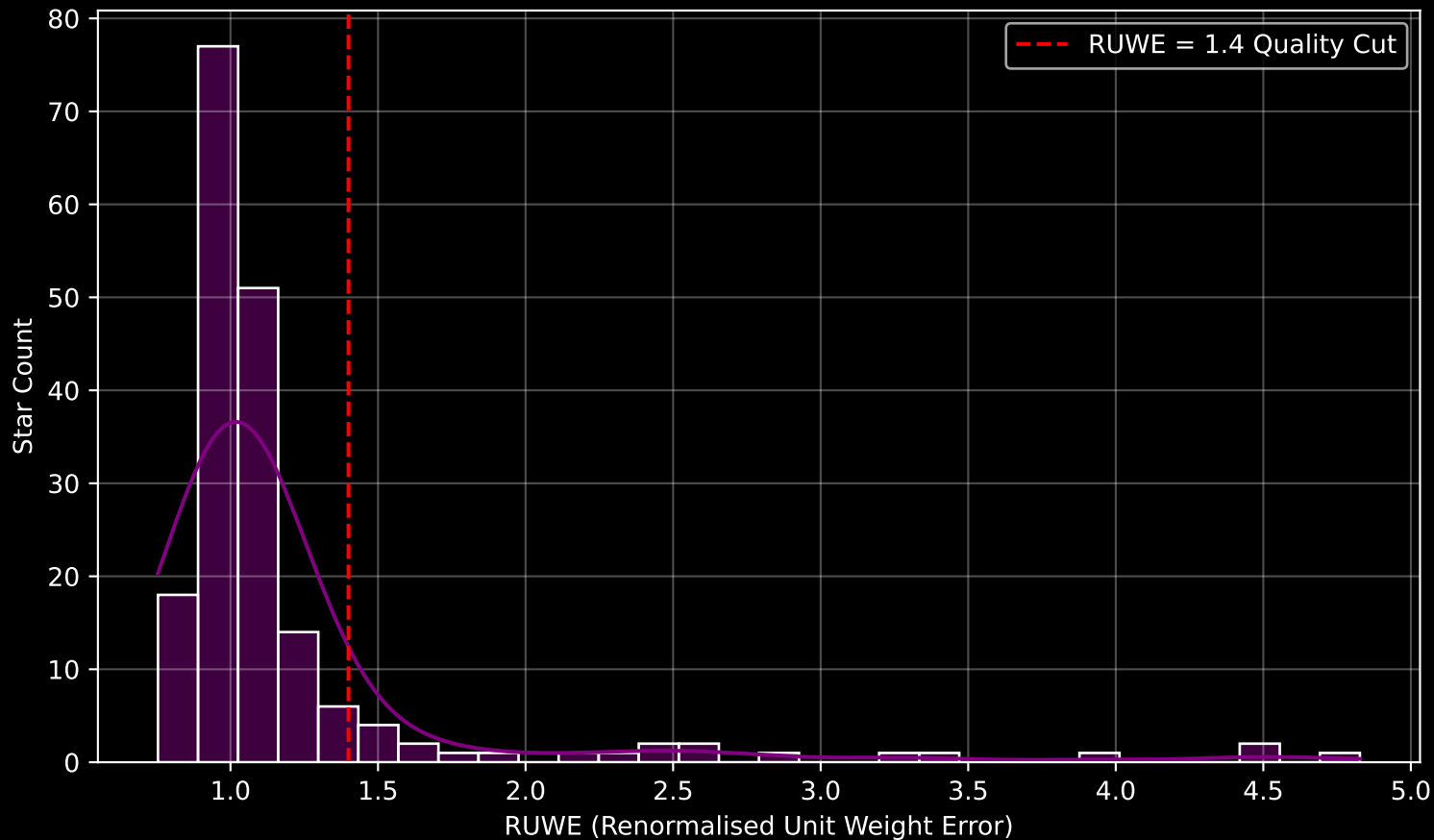
GAPOGEE DR17 Field [261+48] RUWE Distribution (n= 187)
