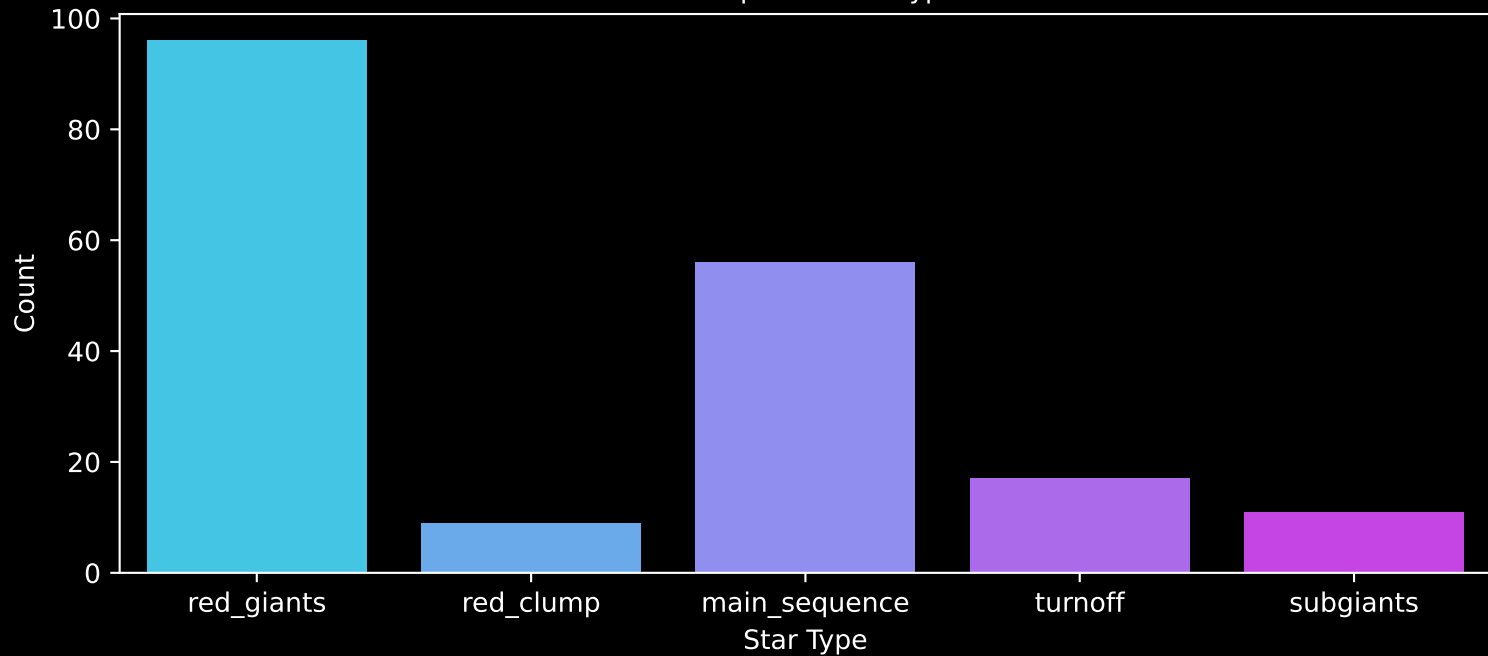
APOGEE DR17 Field: [261+48] Count plot of Star Type
