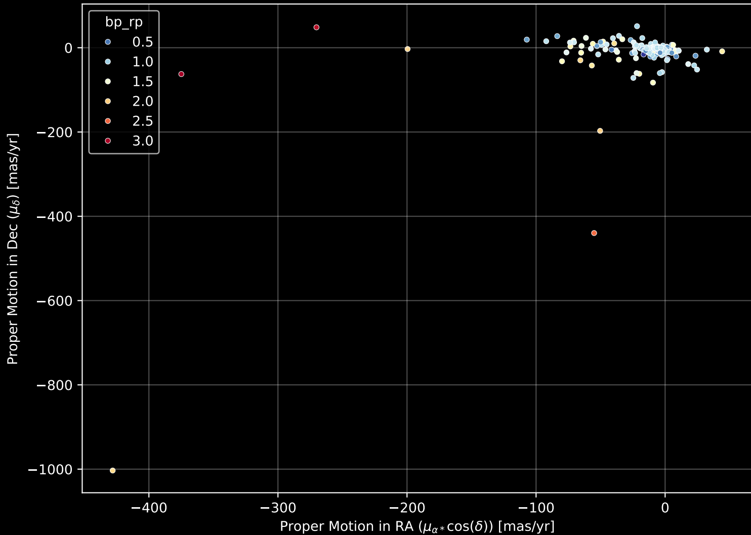
APOGEE DR17 Field: [261+48] Proper Motion Diagram (n= 189)
