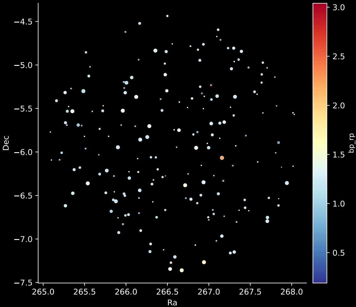
APOGEE DR17 Field: [261+48] Stars: 189
