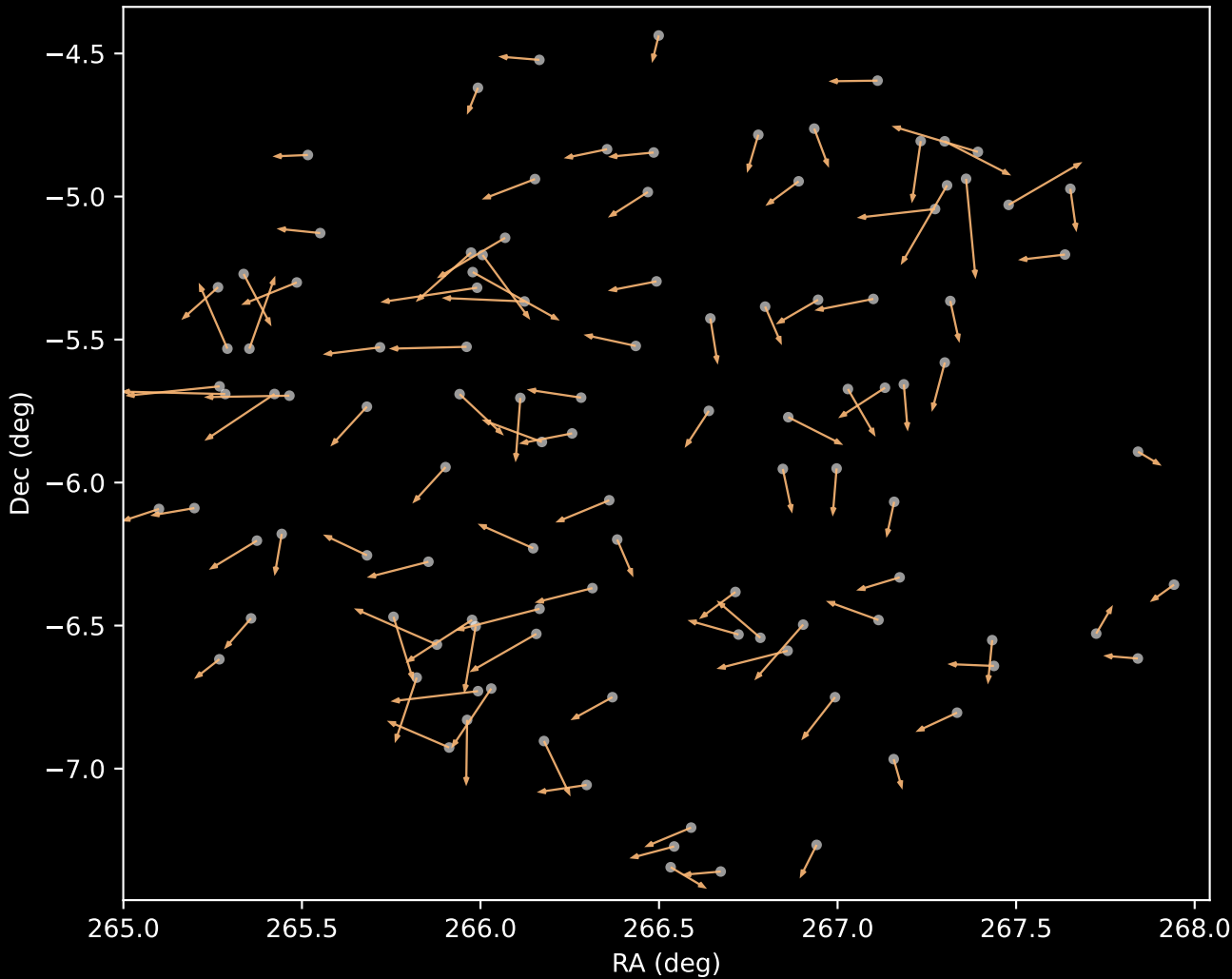
APOGEE DR17 Cluster 3 Proper Motion Vectors (n=109)
