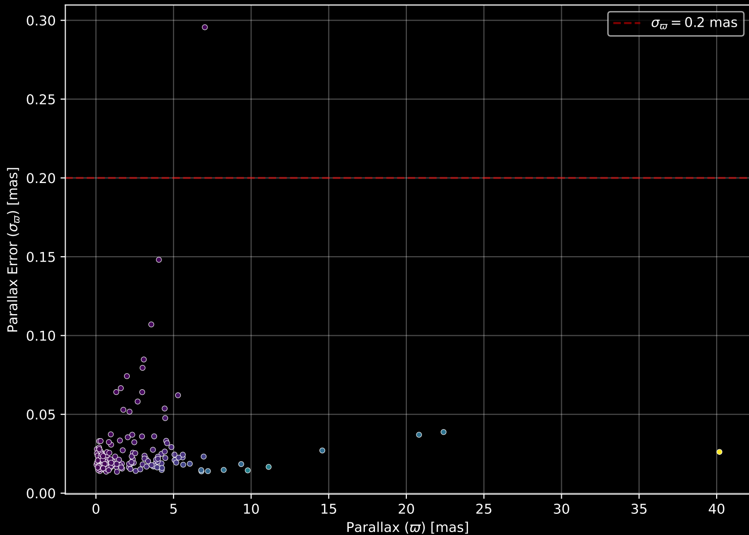
APOGEE DR17 Field: [261+48] Parallax Quality (n= 189)
